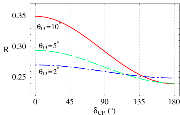
FIG. 2 (color online). Flux ratio R = \phi_\mu^D / (\phi_e^D + \phi_\tau^D) at Earth as a function of \delta_{CP} for \theta_{13} = 10^\circ (red, solid curve), \theta_{13} = 5^\circ (green, dashed curve), and \theta_{13} = 2^\circ (blue, dotted-dash curve); for \theta_{23} = 45^\circ and initial fluxes \phi_e:\phi_\mu:\phi_\tau = 1:0:0 at the source.
