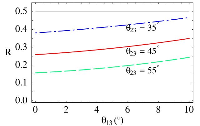
FIG. 1 (color online). Flux ratio R = \phi_e^D / (\phi_\mu^D + \phi_\tau^D) at Earth as a function of \theta_{13} for \theta_{23} = 35^\circ (blue, dotted-dash curve), \theta_{23} = 45^\circ (red, solid curve), \theta_{23} = 55^\circ (green, dashed curve); for initial fluxes \phi_e : \phi_\mu : \phi_\tau = 1:0:0 at the source and \delta_{CP} = 0 . The ratio R = 0.5 expected for standard astrophysical sources is shown for comparison.
