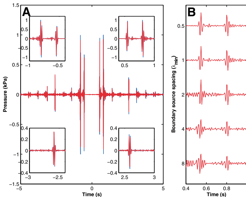
FIG. 3 (color). (a) Waveform computed by summation of the weighted intercorrelation gather shown in Fig. 2 (red) compared to a conventional FD computation (blue). The insets show particular events in the time series. (b) Waveform computed after successive subsampling of the intercorrelation gather.
