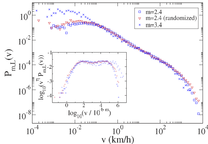
FIG. 3 (color online). The velocity distribution, P_{m,L}(v) , for L = 100 \text{ km} and different values of m : (Blue) crosses and squares correspond to the original data with v_i = \Delta r_i / \Delta t_i . (Red) triangles correspond to a randomization v_i = \Delta r_{\sigma(i)} / \Delta t_i , where \sigma is a randomly chosen permutation of the integers 0 < i < N . Note that \Delta r_i > 2 \text{ km} and \Delta t_i > 60 \text{ s} for all i to avoid any bias due to the uncertainties in the estimates. Inset: Rescaled distributions, using the GR exponent b = 0.95 and \eta = 1.0 .
