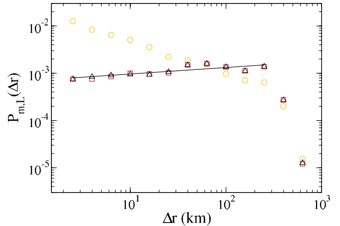
FIG. 2 (color online). The jump distribution, P_{m,L}(\Delta r) , for m = 2.4 and L = 448.5 km. (Orange) circles correspond to the distance between successive earthquakes \Delta r_i = |\mathbf{r}_{i+1} - \mathbf{r}_i| as in Fig. 1. (Red) squares correspond to \Delta r_i = |\mathbf{r}_{\sigma(i+1)} - \mathbf{r}_{\sigma(i)}| where \sigma is a randomly chosen permutation of the integers 0 < i < N , giving a shuffling of the catalog as described in the text. The (black) triangles correspond to the distance between any two earthquakes in the same cell. The solid line is a fit to the latter distribution from 2 to 200 km with a critical exponent of \delta_{\text{shuf}} = -0.14 \pm 0.03 .
