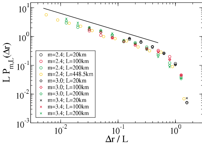
FIG. 1 (color online). Rescaled distribution of jumps, P_{m,L}(\Delta r) , for different values of m and L . L = 448.5 km corresponds to the full area where there is just one cell. Values of \Delta r < 2 km have been discarded due to uncertainties in estimating the epicenters' locations. The solid line with exponent \delta = 0.6 is shown as a guide to the eye.
