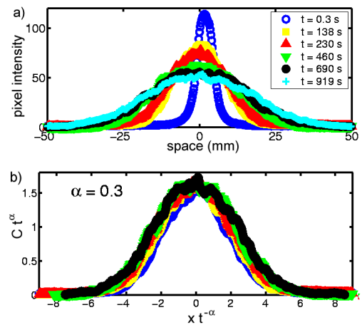
FIG. 3 (color online). (a) Concentration profiles of a mixing pulse of dyed black salt grains surrounded by white salt grains. (b) Collapsed concentration profiles corresponding to (a). The collapse parameter is \alpha = 0.3 .
