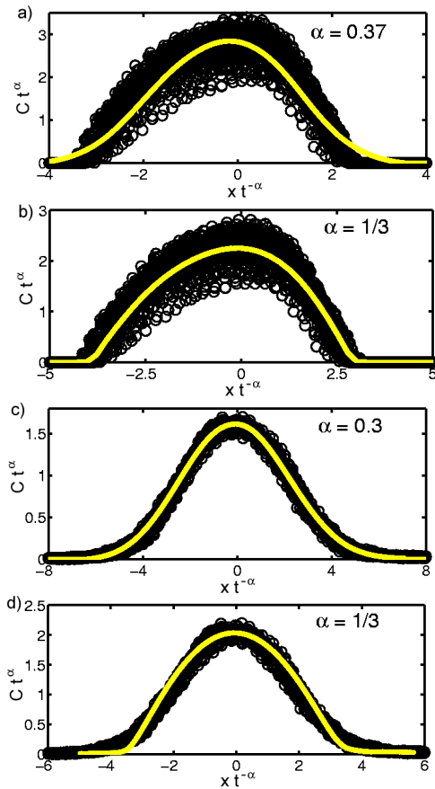
FIG. 4 (color online). Collapsed concentration profiles of a black sand radial core in salt grains fit to (a) the fractional diffusion equation (solid line) and (b) the porous medium equation (solid line). Collapsed concentration profiles of mixing dyed black salt grains fit to (c) the fractional diffusion equation (solid line) and (d) the porous medium equation (solid line).
