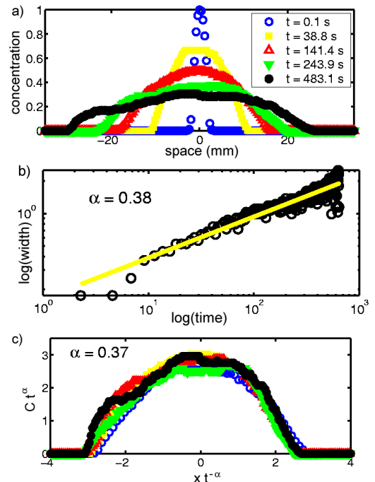
FIG. 2 (color online). (a) Concentration profiles of a spreading radial core pulse of sand grains within salt grains at various times. (b) Power-law scaling of the FWHM of the radial core pulse. From the linear fit (solid line) we find that the width \propto t^{0.38} . (c) Collapsed concentration profiles of the radial core pulse corresponding to (a). The collapse parameter is \alpha = 0.37 .
