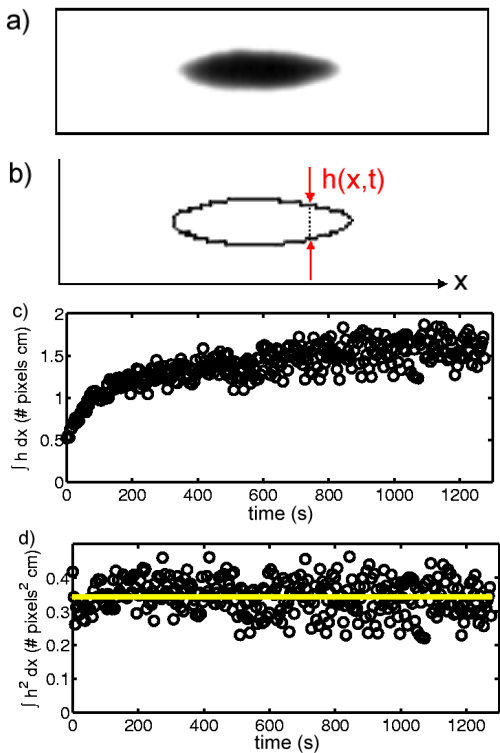
FIG. 1 (color online). (a) An image of the shadow of the radial core formed by 177–212 \mu\text{m} sand grains within 300–420 \mu\text{m} salt grains. (b) The detected edge used to determine the vertical extent h(x, t) of the core. (c) The x integral of h is not constant in time and is thus not proportional to the volume of small grains contained within the radial core. (d) The integral of h^2 is constant in time and is proportional to the desired concentration.
