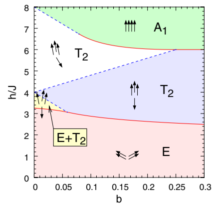
FIG. 2 (color online). Phase diagram as a function of magnetic field h and dimensionless coupling constant b . Solid lines denote first and dashed lines, second order transitions. Spin configurations and irrep of the order parameter in each phase is also shown.
