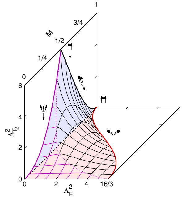
FIG. 4 (color online). Maximal values of the second order invariants \Lambda_E^2 and \Lambda_{T_2}^2 for classical spins as a function of the magnetization per site M . A ridge (dashed line) divides three dimensional from coplanar spin configurations. Spin ordering patterns are shown for the symmetrical cases of \Lambda_E^2 = 0 and \Lambda_{T_2}^2 = 0 .
