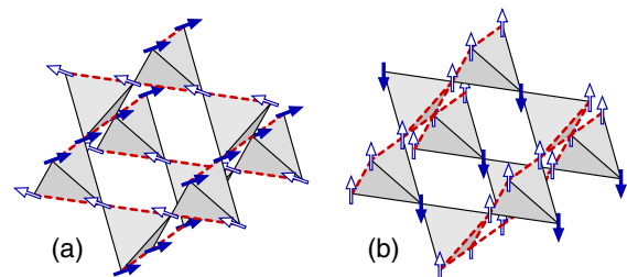
FIG. 1 (color online). A section of the pyrochlore lattice, showing its two-sublattice tetrahedral structure. At zero magnetization, tetragonal lattice distortion favors the spin configurations of the type shown in (a), while at half magnetization trigonal lattice distortion favors the configuration (b). AF bonds are marked with solid black lines and FM bonds with dashed lines.
