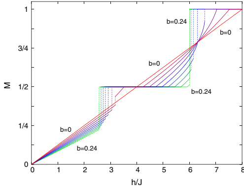
FIG. 3 (color online). Magnetization as a function of magnetic field for b = 0 (straight line) to b = 0.24 (robust plateau) in steps of 0.03.
