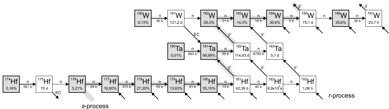
FIG. 1. Nuclear chart of the isotopes of Hf, Ta, and W. Stable isotopes and their relative abundances are shown in shaded squares, whereas the radioactive isotopes and their half-lives are displayed in open squares. Production paths for neutron irradiation are shown as arrows, with labels denoting neutron capture cross sections and decay modes for the radioactive isotopes (data are taken from [4]). The main s process follows the shaded path. The r process is indicated by short arrows.
