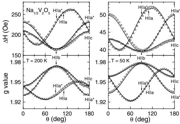
FIG. 3. Angular dependence of ESR linewidth \Delta H and g value of a \beta - \text{Na}_{1/3}\text{V}_2\text{O}_5 single-crystal at 200 K and 50 K (X band). Solid lines: simulations (see text).
