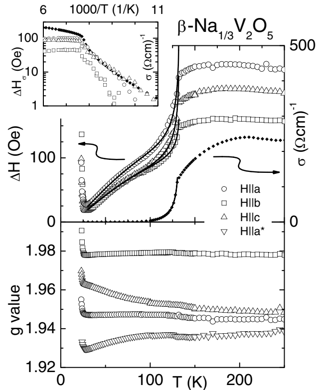
FIG. 2. Temperature dependence of ESR linewidth \Delta H (Inset: reduced contribution \Delta H \sigma compared to b -axis conductivity as Arrhenius plot) and g value of a \beta - \text{Na}_{1/3}\text{V}_2\text{O}_5 single-crystal at Q-band frequency with the external magnetic field parallel to different crystallographic axes.
