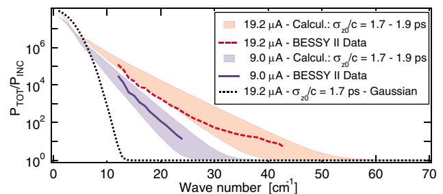
FIG. 2 (color online). CSR gain as a function of the wave number 1/\lambda . The BESSY II data for two different currents per bunch are compared with the shielded SR calculation and with the curve for a Gaussian distribution of the same length.
