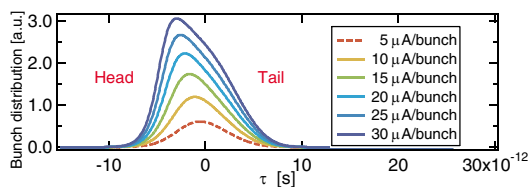
FIG. 1 (color online). Calculated equilibrium longitudinal distribution for different currents per bunch using the shielded SR wake. BESSY II case with a natural bunch length of 2.5 ps.
