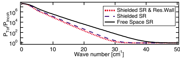
FIG. 3 (color online). CSR gain versus radiation wave number calculated using the shielded SR wake with (dotted line) and without (dashed line) the RW wake. The solid line shows the gain calculated with the FS SR wake. Case of BESSY II with 9.0 \mu\text{A} per bunch and 1.7 \text{ ps} natural bunch length.
