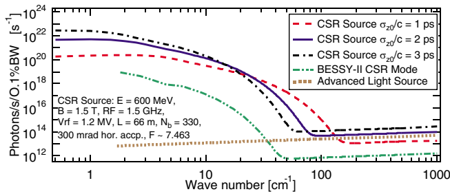
FIG. 4 (color online). Example of source optimized for the CSR production using the criteria described in this Letter. The photon flux is compared with the cases of a conventional SR source (ALS) and of BESSY II CSR mode with 400 bunches, 19.2 \mu\text{A}/\text{bunch} , \sigma_{z0}/c = 1.8 \text{ ps} , and 60 \text{ mrad} horizontal acceptance.
