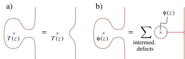
FIG. 1 (color online). A conformal defect is transparent to the stress tensor (a), while a bulk field \phi generically becomes a sum of disorder fields (b).
