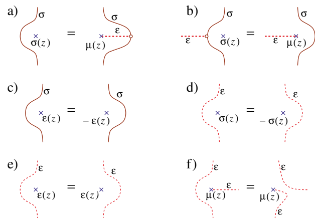
FIG. 3 (color online). Taking defects of type \sigma and \varepsilon past field insertions. The TFT representation of (a) is given in Fig. 2.
