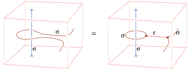
FIG. 2 (color online). The TFT-representation of the pulling a defect of type \sigma past a spin field. Collapsing the circular \sigma -Wilson line on the rhs generates the TFT representation of the disorder field \mu(z) .
