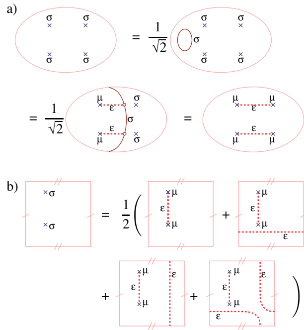
FIG. 4 (color online). Order/Disorder duality of a correlator of four spin fields on a sphere, and of two spin fields on a torus, as induced by the \sigma defect.
