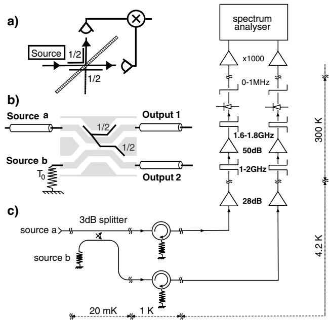
FIG. 1. Schematics of the HBT experiment (a), of the GHz beam splitter (b), of the amplification and detection chains (c). A detailed description is given in the text.
