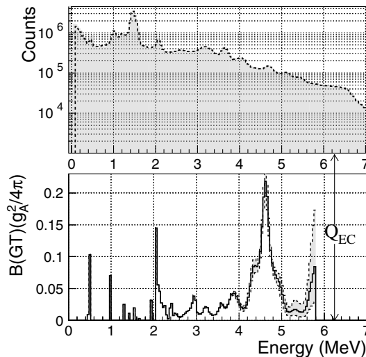
FIG. 1. Upper panel: Experimental total absorption spectrum of the \beta decay of ^{76}\text{Sr} overlaid with the recalculated spectrum after the analysis (see text). Lower panel: B(\text{GT}) distribution derived from the experimental data shown above. The shading represents the experimental uncertainty.
