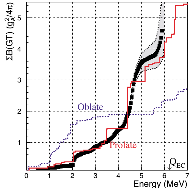
FIG. 2 (color online). Accumulated B(\text{GT}) as a function of the excitation energy in the daughter nucleus. The experimental results from this work (squares) are compared with the theoretical calculations [12] assuming prolate (solid line) and oblate (dashed line) shapes for the ^{76}\text{Sr} ground state. The shading indicates the experimental uncertainty.
