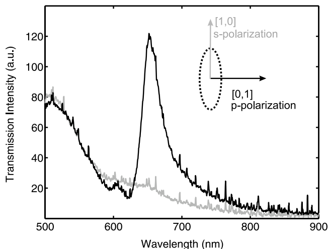
FIG. 2. Transmission spectrum through elliptical nanohole array for two orthogonal linear polarizations, with a 0.3 aspect ratio between the minor and major axes of the ellipse. The p polarization is parallel to the [0, 1] direction.
