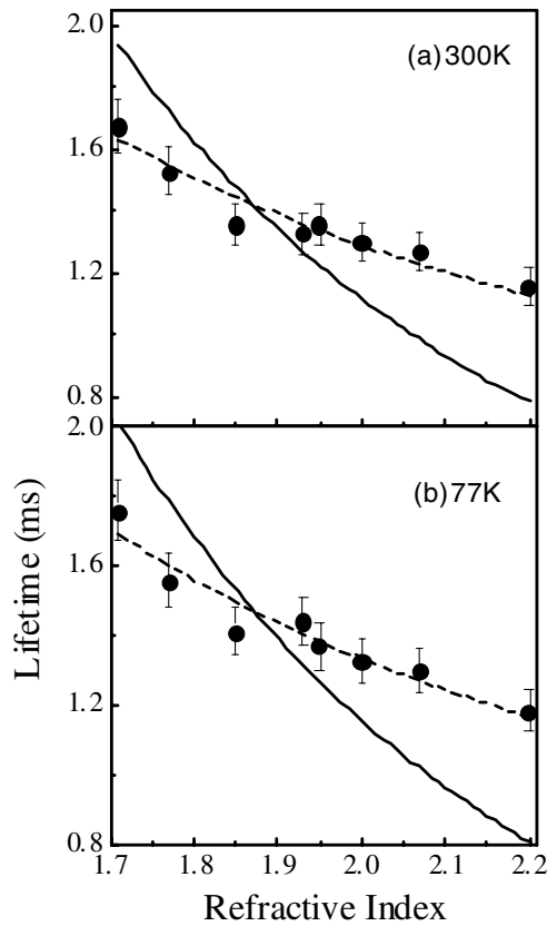
FIG. 2. Lifetimes plotted as a function of the refractive index at (a) 300 K and (b) 77 K. Circles are the experimental data; the dashed lines are the fits for the real cavity and the solid lines for the virtual cavity model.
