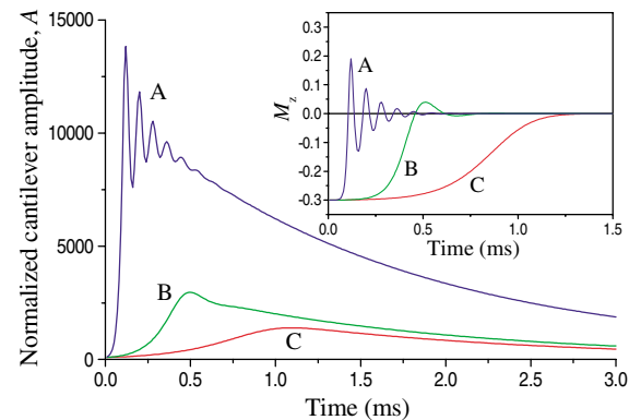
FIG. 2 (color online). Characteristic transients of a cantilaser for different numbers of resonant nuclei within the sensitive slice: (a) N = 200 \times 10^6 , (b) 15 \times 10^6 , and (c) 5 \times 10^6 . The main panel shows the normalized amplitude of cantilever oscillations, A(t) ; the inset shows the longitudinal nuclear polarization, M_z(t) . The initial conditions are A(0) = 94 , M_-(0) = 0 , M_z(0) = -0.3 .
