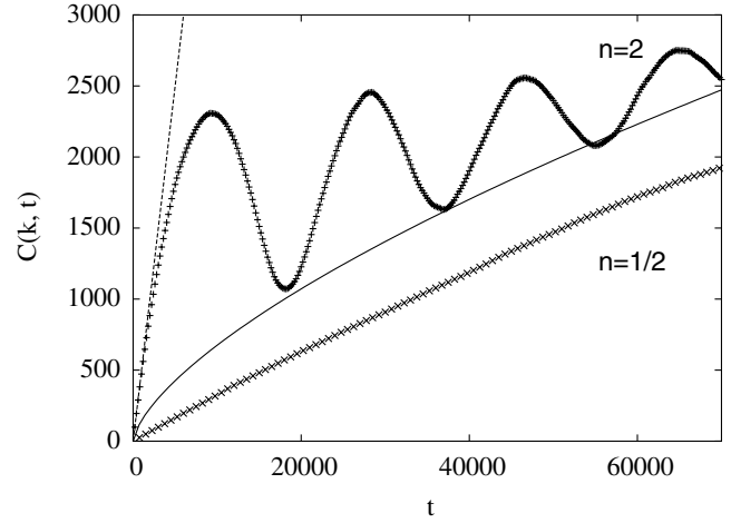
FIG. 1. Plot of the tagged particle correlation C(k, t) vs t at the critical point showing the existence of kinematic waves for n > 1 . For n = 2 , the solid curve passing through the minima is a power law with exponent 2/3 and the initial tangential straight line has a slope equal to c = 1/2 . For n = 1/2 , the y axis has been scaled down by a factor of 15. The data have been averaged over all k for both values of n .
