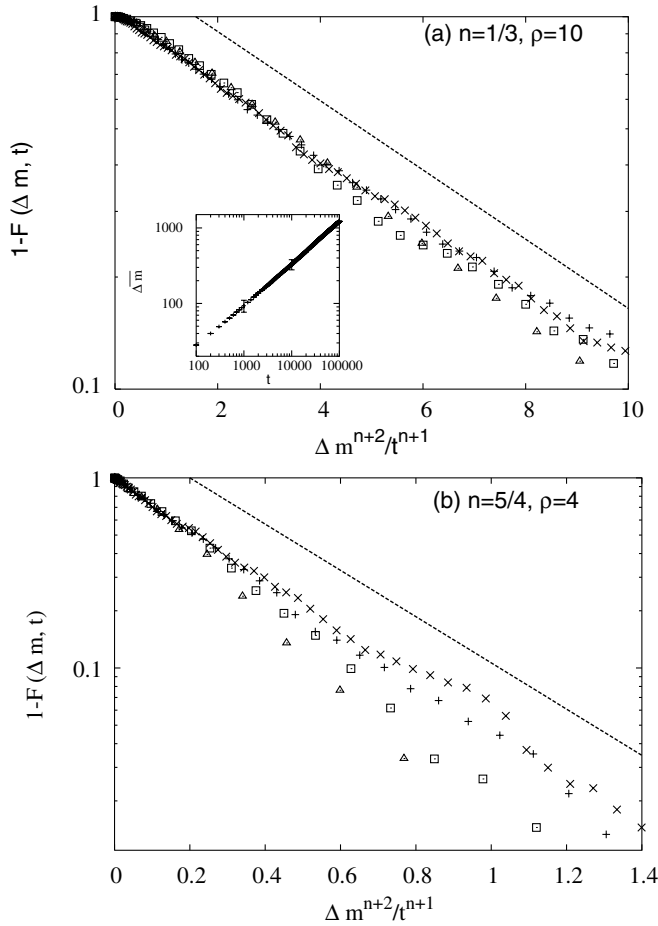
FIG. 2. Scaling collapse of the cumulative distribution in Eq. (8) for (a) n = 1/3 and (b) n = 5/4 at t = 10^4 ( \Delta ), 2 \times 10^4 ( \square ), 4 \times 10^4 ( + ), and 8 \times 10^4 ( \times ) in the condensate phase. The data are obtained from the two slowest sites in 150 disorder configurations, using c = 1/2 . The broken line is a guide to the eye. The inset shows the temporal growth of average mass as a power law with exponent \beta given in the text.
