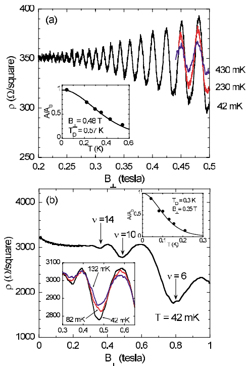
FIG. 1 (color online). Shubnikov-de Haas (SdH) oscillations in sample NH50.3064.9N at n_s = 7.3 \times 10^{11} \text{ cm}^{-2} (a) and n_s = 1.17 \times 10^{11} \text{ cm}^{-2} (b). The vertical arrows in (b) show the positions of the SdH minima corresponding to Landau filling factors \nu = 14, 10, and 6 as labeled. Temperatures are indicated in the figures. Measuring current is 2 nA (a) and 200 pA (b). The experimentally measured amplitudes of the oscillations are shown in the insets by solid circles together with the calculated dependences (solid lines); the parameters used in calculations are indicated in the insets. The lower inset in (b) shows a close-up view of two SdH oscillations corresponding to \nu = 14 and 10 measured at three temperatures.
