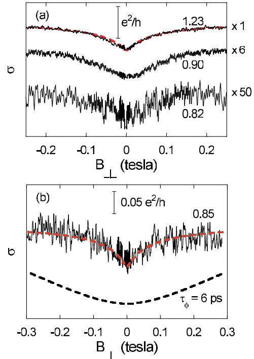
FIG. 3 (color online). Magnetoconductivity in sample NH50.3064.9N at T = 42 mK and at different electron densities indicated near the curves in units of 10^{11} \text{ cm}^{-2} . (a) The curves are vertically shifted for clarity, and two lower curves are multiplied by 6 (the middle one) and 50 (the lower one), which makes them quantitatively similar to the upper (unmodified) curve. The thick dashed line is the fit by Eq. (1) with \alpha = 0.6 and \tau_{\phi} = 30 ps. (b) Unsuccessful attempt to fit the experimental data for n_s = 0.85 \times 10^{11} \text{ cm}^{-2} by Eq. (1) with the same prefactor \alpha = 0.6 as above but reduced \tau_{\phi} = 6 ps (the lower dashed curve, which is shifted for clarity). However, the data can be fitted reasonably well by choosing \tau_{\phi} = 30 ps as in (a), but with the prefactor 10 times smaller ( \alpha = 0.06 ; the upper dashed curve).
