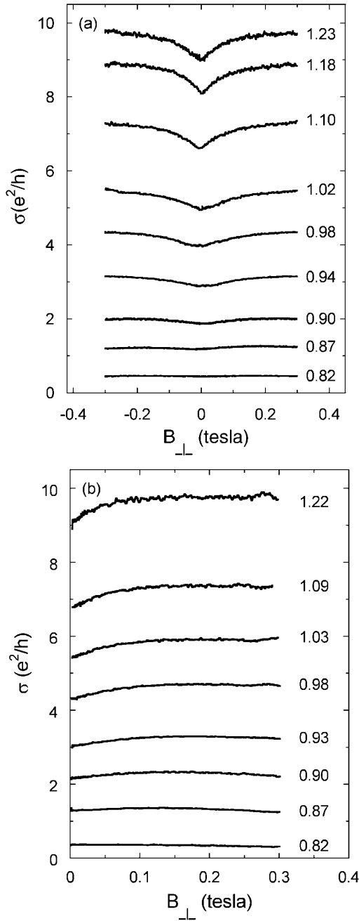
FIG. 2. Longitudinal magnetoconductivity in a weak perpendicular magnetic field at T = 42 mK for a range of electron densities which are indicated near each curve in units of 10^{11} \text{ cm}^{-2} in samples NH50.3064.9N (a) and NH50.4064.7N (b).
