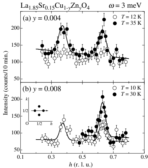
FIG. 1. q profiles along the h direction through (\pi, \pi) at the transfer energy \omega = 3 meV for (a) y = 0.004 and (b) y = 0.008 below (open circles) and above (solid circles) T_c .
