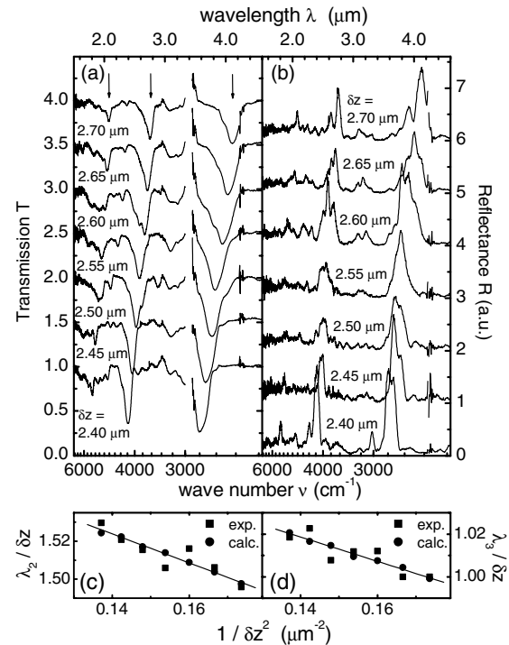
FIG. 3. Higher-order bandgaps in transmission (a) and reflection (b) for constant \delta z/\delta x = 2.0 with layer spacing \delta z varying from 2.4 to 2.7 \mu\text{m} . Dips in transmission correspond to spikes in reflection. (c) First and (d) second higher-order gap wavelengths as a function of \delta z with linear curve fit and photonic band theory results.
