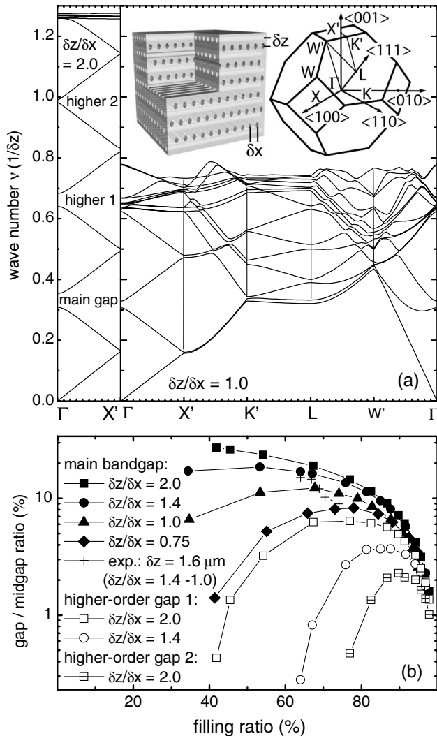
FIG. 1. (a) Photonic band structures of woodpile-type polymer void channel photonic crystals for ratios \delta z/\delta x of 1.0 (right) and 2.0 (left, only \Gamma X' ), as calculated for \delta z = 2.5\text{ }\mu\text{m} and elliptical channel cross section of diameters 750 nm and 1.125 \mu\text{m} . The number of higher-order gaps strongly depends on \delta z/\delta x . Inset: Geometrical arrangement of void channels and corresponding first Brillouin zone. (b) Dependence of the gap/midgap ratio on the filling ratio for various values of \delta z/\delta x .
