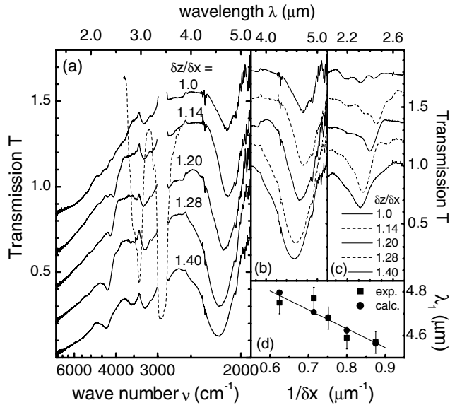
FIG. 2. Infrared spectra of woodpile structures at constant \delta z = 1.6 \mu\text{m} with \delta x varying from 1.14 to 1.6 \mu\text{m} . (a) As measured; dashed line: polymer absorption. (b) Fundamental photonic band gap and (c) first higher-order gap after baseline correction. (d) Linear dependence of the gap wavelength on the inverse in-plane channel spacing.
