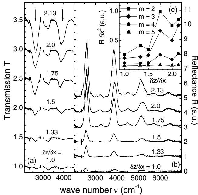
FIG. 4. (a) Transmission and (b) reflection infrared spectra at constant \delta z = 2.55 \mu\text{m} and varying unit cell geometry ( \delta z/\delta x = 2.13-1.0 ). Note the emergence of higher-order band gaps ( m = 2, 3 ) with increasing \delta z/\delta x . (c) Calibrated peak reflectances reveal the transformation of Bragg resonances into photonic band gap reflections.
