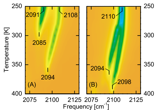
FIG. 1 (color online). Pseudo-3D plot of IR spectra obtained after heating saturated CO layers on Pt/Ru(0001) films (adsorbed at 80 K) to the indicated temperatures (ordinate) and recooling to 100 K. In panel (a) 1.3 ML Pt have been deposited; in panel (b) this value has been increased to 2.5 ML. The observed frequency shifts are attributed to thermal desorption of CO. The color is indicating the reflectivity change from 0% (red) to 10% (blue) with the edges of the peaks clearly visible as yellow (or light gray, respectively) contours.
