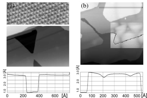
FIG. 2. STM images of bimetallic Pt/Ru(0001) layers grown at T_G = 600 \text{ K} at a rate R = 5 \times 10^{-4} \text{ ML/s} . (a) Topography ( 800 \text{ \AA} \times 530 \text{ \AA} ) and line scan ( l = 780 \text{ \AA} ) of a 4 ML Pt film; also shown is an enlarged area ( 50 \text{ \AA} \times 17 \text{ \AA} ) displaying the hexagonal lattice of the pseudomorphic Pt layers. (b) Topography ( 800 \text{ \AA} \times 800 \text{ \AA} ) and line scan ( l = 550 \text{ \AA} ) of an 8 ML Pt film. Apparently, dislocation lines are formed for 8 ML Pt films while they are absent at 4 ML. The gray scale within the rectangular area ( 420 \text{ \AA} \times 330 \text{ \AA} ) has been adjusted to improve the visibility of the dislocations.
