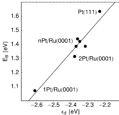
FIG. 4. CO binding energy, E_B , for a p(2 \times 2) -CO ordered overlayer versus d -band center, \epsilon_d (with respect to the Fermi energy) of the surface Pt atom. The solid line represents the best least-squares linear fit.
