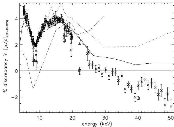
FIG. 2. Discrepancies in the total mass attenuation cross section of silicon between experiments from Gerward [30] ( \diamond ), Creagh [4,28] ( \square ), Baltazar-Rodrigues et al. [31] ( \triangle ), Mika et al. [5] ( \times ), and this work ( \bullet ). All theoretical curves are for ideally misaligned crystalline silicon. Theoretical predictions of total cross sections are therefore the sum of PE, Compton, and TDS components. Theoretical tabulations are presented from Chantler [12] (solid line), XCOM [27] (dotted line), Scofield [16] for PE, Hubbell et al. [33] for Compton, and Chantler for TDS), Henke et al. [10] (dot-dashed line, using Chantler for TDS), Creagh [11] (dashed line, using Chantler for TDS), and Kissel [35] (dot-dot-dot-dashed line, using Chantler for Compton and TDS). Agreement with theory is much improved.
