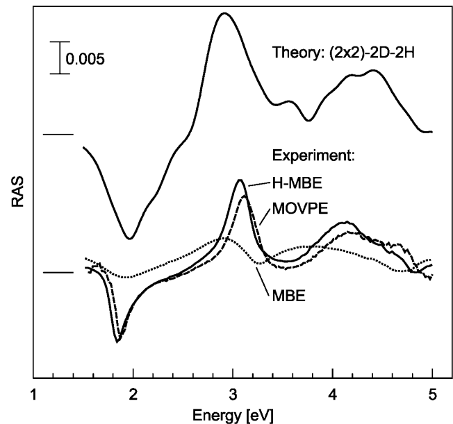
FIG. 4. RAS spectra [\text{Re}\{(r_{[110]} - r_{[110]})/(r)\}] measured for P-terminated InP(001) (2 \times 1) surfaces prepared by MBE, by MBE with additional hydrogen supply, and by MOVPE (from Ref. [23]) are compared with the spectrum calculated for the InP(001) (2 \times 2) -2D-2H structure (cf. Fig. 1).
