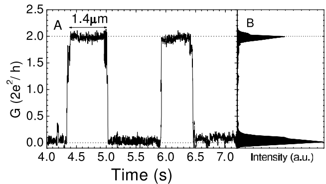
FIG. 1. A sequence of measurements of conductance versus time showing steps at 2G_0 , where G_0 is the conductance quantum G = 2e^2/h . Two steps of different lengths out of a sequence of more than fifty are shown. The histogram shows the persistence of the quantized value along the sequence, with a clearly defined peak at 2G_0 . The bias voltage between tip and substrate was V_p = 10 \text{ mV} .
