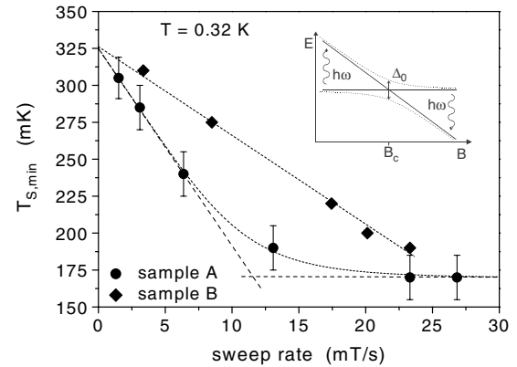
FIG. 3. Dependence of the minimal spin temperature T_{s,\min} on the field sweep rate for two samples. Dashed lines are guides to the eye. The inset schematically presents the two states at the level crossing and indicates the splitting \Delta_0 discussed in the text.
