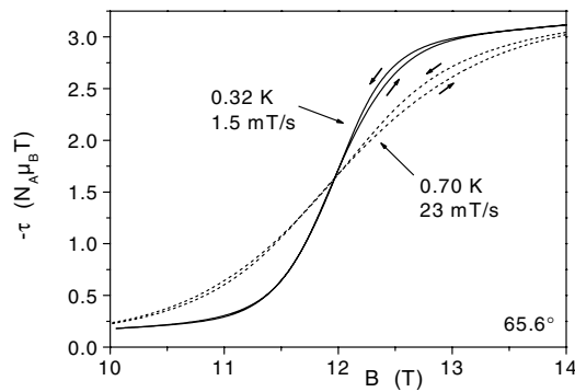
FIG. 4. Two example curves showing the asymmetry of the hysteresis loop around B_c discussed in the text.
