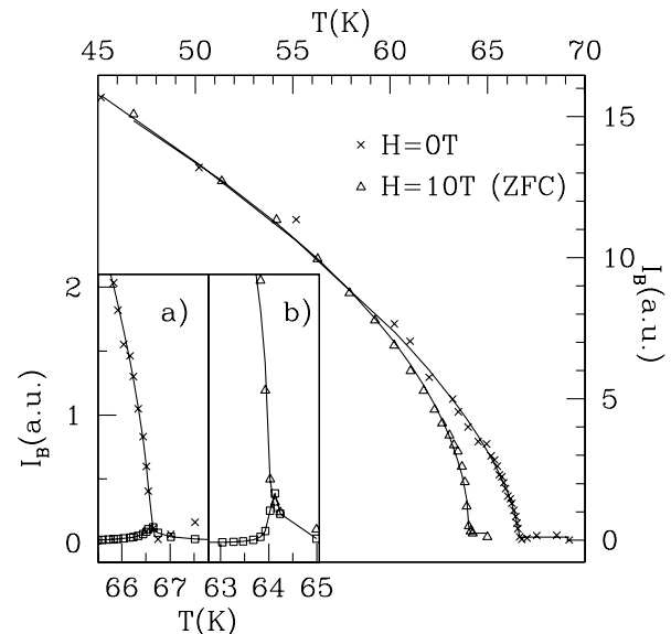
FIG. 1. The ZFC Bragg intensity, I_B , in arbitrary units (a.u.), versus T for H = 0 and H = 10 T, with the T -independent background intensity subtracted. The square symbols in insets (a) and (b) show the critical scattering contributions to the x-ray intensities for H = 0 and H = 10 T, respectively, determined from neutron scattering measurements as described in the text.
