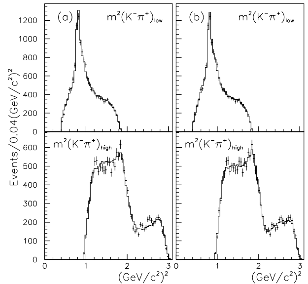
FIG. 2. m^2(K\pi)_{\text{low}} and m^2(K\pi)_{\text{high}} projections for data (error bars) and fast-MC (solid line): Models A (a) and C (b).
