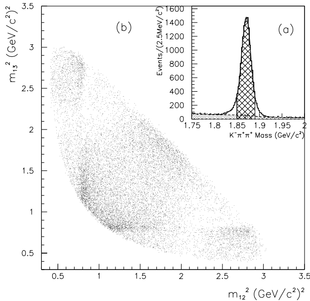
FIG. 1. (a) The K^- \pi^+ \pi^+ invariant mass spectrum. The shaded area corresponds to the background level. The cross-hatched region is the sample used for the Dalitz-plot analysis. (b) The D^+ \rightarrow K^- \pi^+ \pi^+ Dalitz-plot, symmetrized for the indistinguishable pions.
