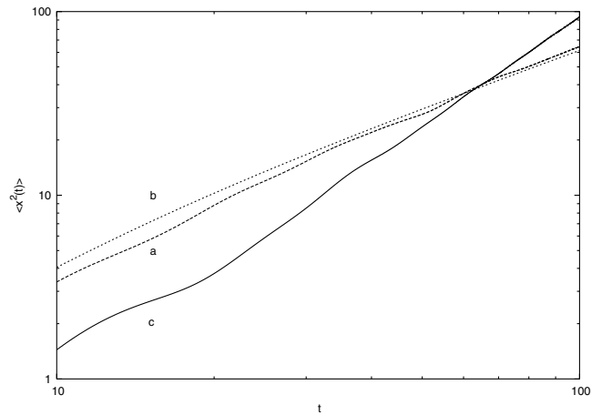
FIG. 2. \langle x^2(t) \rangle vs t . Curve (a) shows a simulation of the GLE, with \omega_S = 0.5 and a NDS given in Eq. (18), while curve (b) is for the system without memory. Curve (c) shows a simulation of the GLE with a NDS given in Eq. (22), with \omega_1 = \omega_S/2 . In this case we find superdiffusive behavior.
