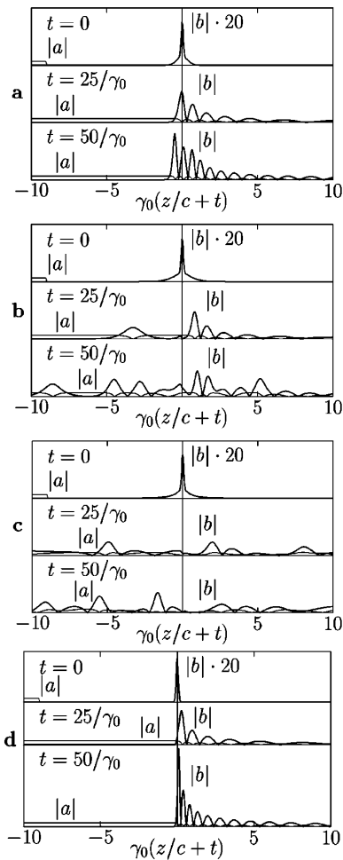
FIG. 1. For exactly resonant BRA, evolution of a short Gaussian seed accompanied by a longer prepulse of (a) Gaussian, (b) hyperbolic secant, and (c) Lorentz form. For comparison, (d) no prepulse.
