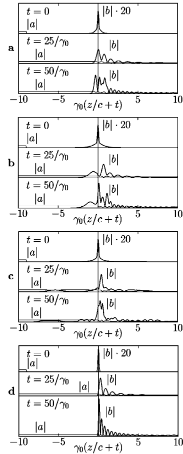
FIG. 2. Under detuning q = 0.25 , evolution of the short Gaussian seed accompanied by a longer prepulse seed of (a) Gaussian, (b) Poisson, and (c) Lorentz form. For comparison, (d) no prepulse.
