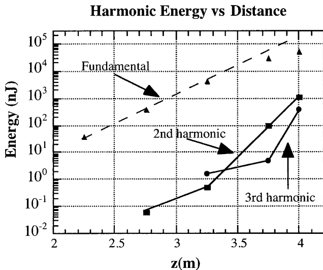
FIG. 2. Energy vs distance for the fundamental, 2nd and 3rd harmonics. The gain lengths for these are 19, 9.8, and 6.0 cm, respectively.
