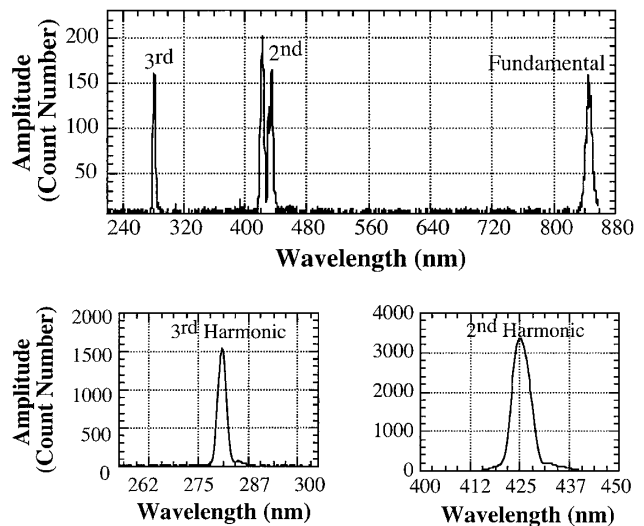
FIG. 1. (a) Single shot harmonic spectra of the fundamental, 2nd and 3rd harmonics. (b) Harmonic spectra independently measured at peak VISA gain.
