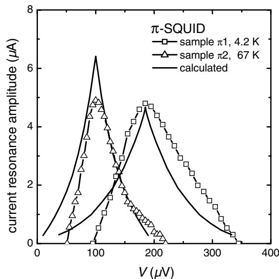
FIG. 4. Zero-field resonance current I_{lr} as a function of voltage for the two \pi SQUIDs at different temperatures.
