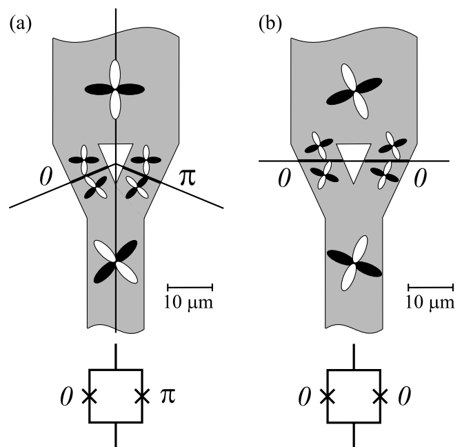
FIG. 1. Schematics of (a) the \pi SQUIDs and (b) the standard SQUID investigated. For both, the junctions straddle symmetric 45^\circ [001] tilt boundaries (from [8]).
