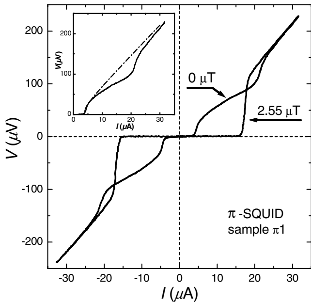
FIG. 2. Current-voltage characteristics measured at 4.2 K of a \pi -SQUID at zero field and for the smallest magnetic field which causes a maximum of I_c . The inset shows a measured characteristic together with a fit based on the RSJ model.
