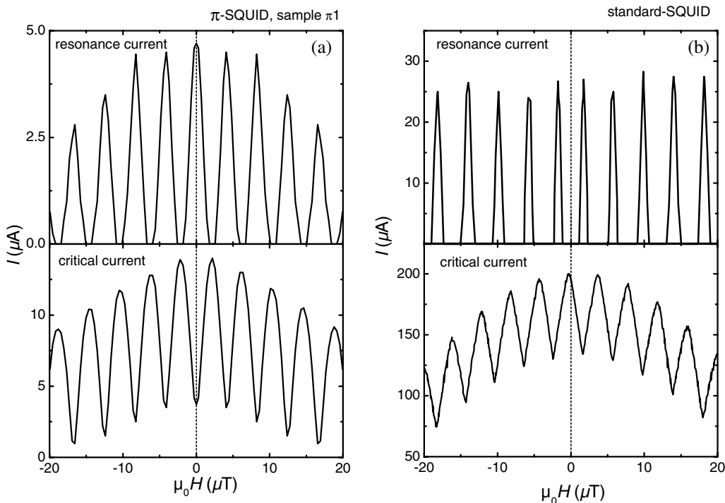
FIG. 3. Dependencies of the maximum resonance current I_r and of the critical current I_c at 4 K of (a) a \pi SQUID and (b) the standard SQUID as a function of applied magnetic field.
