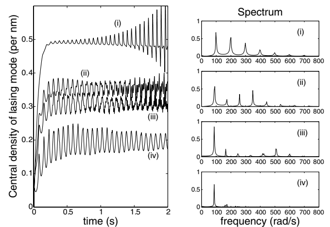
FIG. 2. Time series and power spectra of the laser mode central density. The pumping rate is R = 10^5 \text{ s}^{-1} . The scattering lengths are (i) a_{tt} = 0.01 \text{ nm} , (ii) a_{tt} = 0.5 \text{ nm} , (iii) a_{tt} = 1 \text{ nm} , and (iv) a_{tt} = 10 \text{ nm} . Spectral power is in arbitrary units and is obtained from the time series after the initial 0.4 s.
