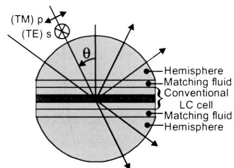
FIG. 1. Hemispheres are used for coupling a convergent beam into and out of fully leaky guided modes that are resonant within the liquid crystal layer of a commercially fabricated cell.
