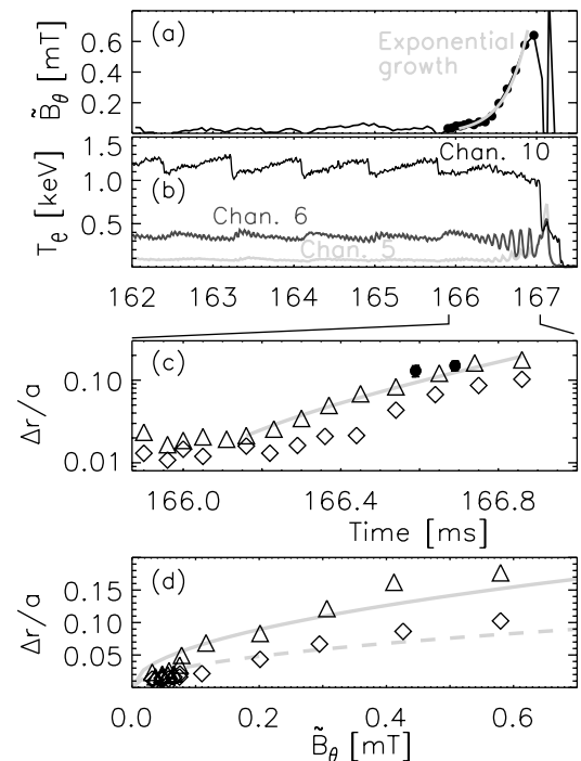
FIG. 1. (a) Amplitude of \tilde{B}_\theta . (b) ECE T_e in the center (channel 10) and in the vicinity of the q = 2 surface (channels 6 and 5) [see Fig. 2(a)]. (c) \Delta r/a calculated with (4). The solid circles indicate the island width estimated from TS [see Figs. 2(c)–2(e)]. The gray line is the fit to Eq. (10). (d) \Delta r/a plotted against \tilde{B}_\theta . The dashed (solid) gray line represents Eq. (6) [Eq. (5)]. Symbol \Delta ( \diamond ) refers to LFS (HFS).
