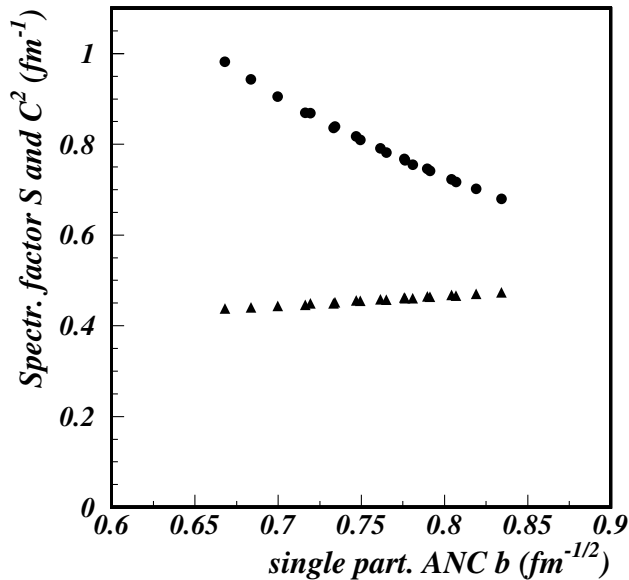
FIG. 2. Comparison of the spectroscopic factors S_{\text{tot}} (dots) and of the ANC C_{\text{tot}}^2 (triangles) extracted from the ^8\text{B} breakup data on Si at 38 MeV/u [10], for different parameters of the single particle Woods-Saxon potentials.
