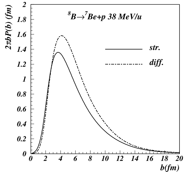
FIG. 1. The stripping and diffraction dissociation parts of the breakup probability as a function of the impact parameter.
