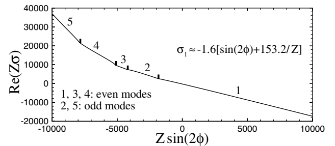
FIG. 2. The real part of the most unstable eigenvalue \sigma for an elastic filament in the plane of shear at a given dimensionless flow strength Z and azimuthal angle \phi .
