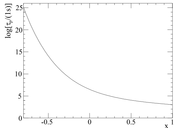
FIG. 1. T_p \equiv \log_{10}[\tau_p/(1 \text{ s})] is plotted as a function of x \equiv \log_{10}[a/(1 \text{ MeV})] , where \tau_p is the p^+ mean proper lifetime, a its proper acceleration, m_e = 0.511 \text{ MeV} , and \Delta m = 1.29 \text{ MeV} . ( 1 \text{ MeV} \approx 4.6 \times 10^{31} \text{ cm/s}^2 .) Note that \tau_p \rightarrow +\infty for inertial p^+ 's.
