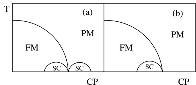
FIG. 1. Schematic phase diagram showing the paramagnetic (PM), ferromagnetic (FM), and superconducting (SC) phases in a temperature ( T )-control parameter (CP) plane. (a) The qualitative prediction of paramagnon theory [5], and (b) the qualitative phase diagram as observed in \text{UGe}_2 [3] and explained by the theory presented here. In Ref. [3], hydrostatic pressure serves as CP.
