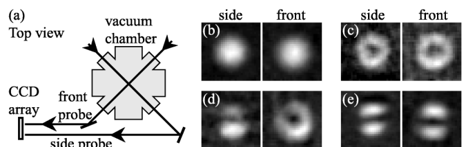
FIG. 3. (a) An illustration of our probe beam paths. (b)–(e) Simultaneous 100- \mu\text{m} -square images of trapped condensates from the front and side imaging directions. Shown are (b) a ground state condensate of component |1\rangle , (c) a shell of |1\rangle atoms around a central ball of |2\rangle atoms [21,22], (d) a |1\rangle vortex filled with |2\rangle atoms, and (e) a horizontally oriented dark soliton of component |1\rangle , filled with |2\rangle atoms.
