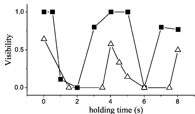
FIG. 3. Visibility of a vortex in a BEC is plotted versus the time the BEC is held in a trap squeezed along an axis at 45^\circ to the line of sight. Visibility is the probability of detecting a vortex over several shots. Solid squares indicate vortex detection with the surface-wave technique; open triangles indicate detection with the expansion technique.
