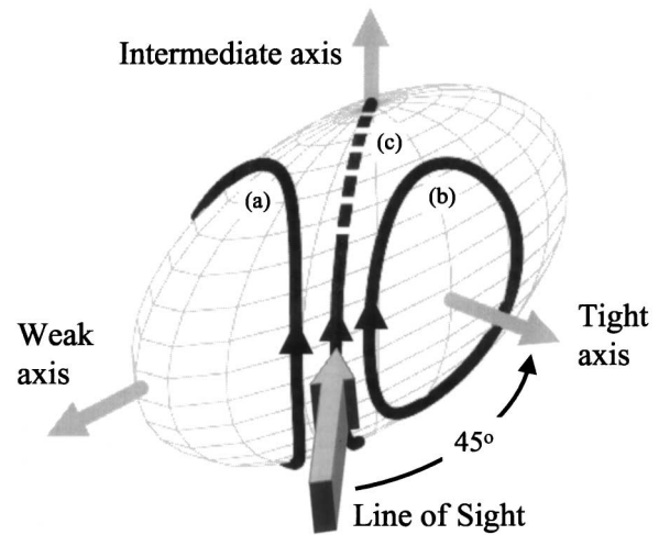
FIG. 2. Possible tilting behavior of a vortex in a confined BEC is illustrated for the conditions of the second tilting experiment (see text). The axes of symmetry for the triaxial confining potential are indicated. Initially, the vortex is nearly antialigned with the line of sight. Depending on the precise initial orientation of the vortex and the relative values of the confinement strengths, the vortex direction could (a) precess about the weak axis, (b) precess about the tight axis, or (c) drift towards the intermediate axis along a "saddle" line, as traced out on the surface of the condensate.
