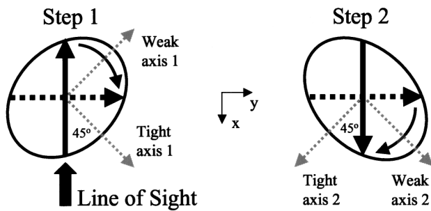
FIG. 4. A sequence of trap deformations to reverse the direction of a vortex is shown. The figure shows a horizontal cross section of the BEC as seen from above. The vortex is initially formed along the line of sight and aligned with the -\hat{x} axis. In step 1, the trap is squeezed in the horizontal plane along tight axis 1. The vortex is then allowed to precess for 1.5 s, at which point it should be aligned with the \hat{y} axis. The new direction of the vortex is indicated by a dotted arrow. In step 2, the trap is squeezed along tight axis 2 and the vortex allowed to precess another 1.5 s until it is aligned with the \hat{x} axis. To an observer looking down the line of sight, the vortex has effectively reversed its handedness. Changing the time allowed for vortex precession by 0.5 s inhibited the effect. For the correct timing, the flipping process was found to be successful 80% of the time.
