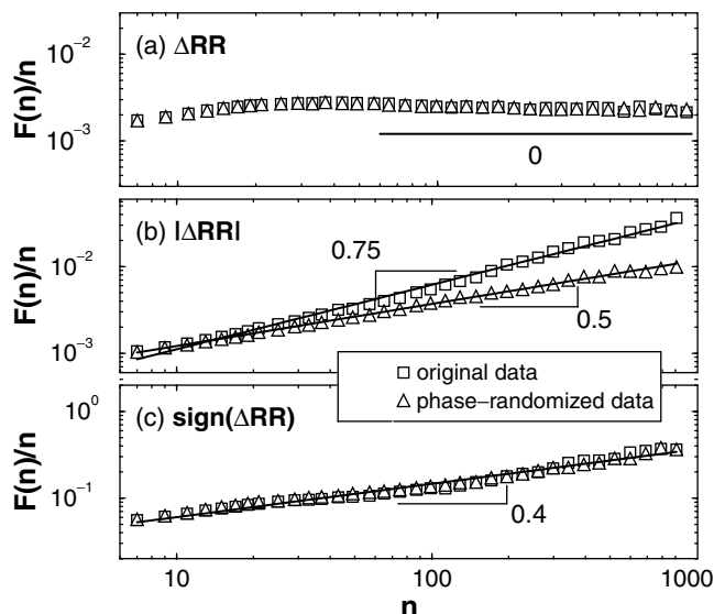
FIG. 2. (a) Root mean square fluctuation, F(n) , for \approx 6 hour record ( \approx 32\,000 data points) for the interbeat interval RR_i series ( \square ) of healthy subject [9]. Here, n indicates the time scale (in beat numbers) over which each measure is calculated. The scaling is obtained using second order detrended fluctuation analysis, and indicates long-range anticorrelations in the heartbeat interval increment series \Delta RR_i [6]. As expected, the scaling properties of the heartbeat interval increment series remain unchanged after the Fourier phase randomization ( \triangle ). (b) The root mean square fluctuation of the integrated magnitude series |\Delta RR_i| [ \square ] indicates long-range correlations in the magnitude series [ \square ] [group average exponent of \alpha - 1 = 0.74 \pm 0.08 where F(n)/n \propto n^{\alpha-1} ]. After Fourier phase randomization of the interbeat interval increment series we find random behavior with exponent 0.5 ( \triangle ). This change in the scaling (after removing the nonlinear features in the time series) suggests that the magnitude series carries information about the nonlinear properties of the heartbeat dynamics. (c) The root mean square fluctuation of the integrated sign series ( \square ) indicates anticorrelated behavior in \text{sign}(\Delta RR_i) [group average exponent of \alpha - 1 = 0.42 \pm 0.03 where F(n)/n \propto n^{\alpha-1} ]. The scaling properties of the sign series remain unchanged after the Fourier phase randomization ( \triangle ), which suggests that the sign series relates to linear properties of the heartbeat interval time series. We note the apparent crossovers at n \approx 20 beats and n \approx 100 beats. A gradual loss of anticorrelation in the sign series is observed at time scales larger than n \approx 100 beats. We note, however, that heartbeat increments derived from the original time series are anticorrelated up to scales of thousands of heartbeats.
