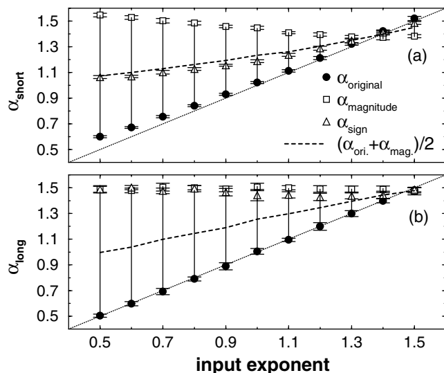
FIG. 4. (a) The relation between the scaling exponents of correlated noise, the integrated magnitude series, and the integrated sign series for the short-range regime ( n < 16 ). We generate 10 series of length 32768 with different correlations (input exponent) and then calculate the scaling exponents of the original series ( \bullet ), of the integrated magnitude series ( \square ), and of the integrated sign series ( \triangle ). In the figure we show the average \pm 1 standard deviation. The dashed line indicates the approximate empirical relation between the different scaling exponents [ \alpha_{\text{sign}} \approx (\alpha_{\text{original}} + \alpha_{\text{magnitude}})/2 ]. This empirical approximation is good for the short-range regime only ( n < 16 ). (b) Same as (a) for the long-range regime ( n > 64 ). Here the approximation does not hold anymore. In this regime the scaling exponents of the magnitude and sign series are uncorrelated no matter what is the exponent of the original series.
