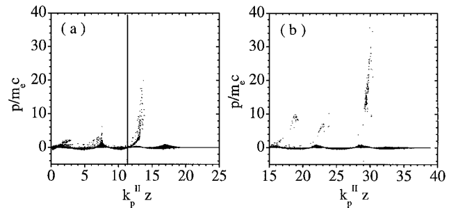
FIG. 2. Longitudinal momentum versus z of the plasma electrons for Figs. 1(a) and 1(b).
