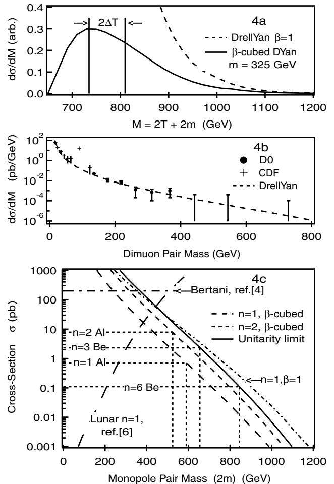
FIG. 4. Cross section plots. (a) d\sigma/dM for Drell-Yan production. The solid curve, cut between the two kinetic energy ( T ) limits, yields the acceptance for stopping and trapping n = 1 monopoles in the aluminum extension cylinder. The dashed curve gives that for dimuons. (b) The differential dimuon cross section is normalized to the D0 [21] and CDF [20] dimuon data. (c) The d\sigma/dM curve of (b) is multiplied by \beta^3 , integrated and renormalized by a factor of n^2(137/2)^2 to give the ‘‘canonical’’ cross section curves versus pair mass ( 2m ) as shown. For the lunar samples, the ordinate is the proton-nucleon cross section. The n = 1, \beta = 1 curve is shown for comparison because the \beta^3 correction was not included in previously published limits. Here, for comparison, the lunar limit from Ref. [6] is shown, where the curve gives the upper limit to the cross section for a given monopole pair mass.
