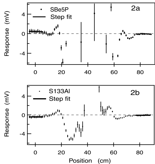
FIG. 2. Sample spectra. (a) Beryllium sample "SBe5P," and (b) aluminum sample "S133Al." The observed steps are -0.8 mV in (a) and +0.4 mV in (b). The dipole signals are off scale in the middle regions of the plot in this vertically expanded view.
