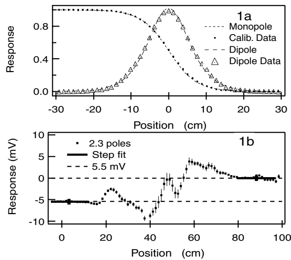
FIG. 1. "Pseudopole" curves. (a) Comparison of theoretical monopole response to an experimental calibration and of a simple point dipole of one sample with that calculated from the theoretical response curve. (b) The observed "step" for a pseudopole current, corresponding to 2.3 minimum Dirac poles, embedded in an Al sample.
