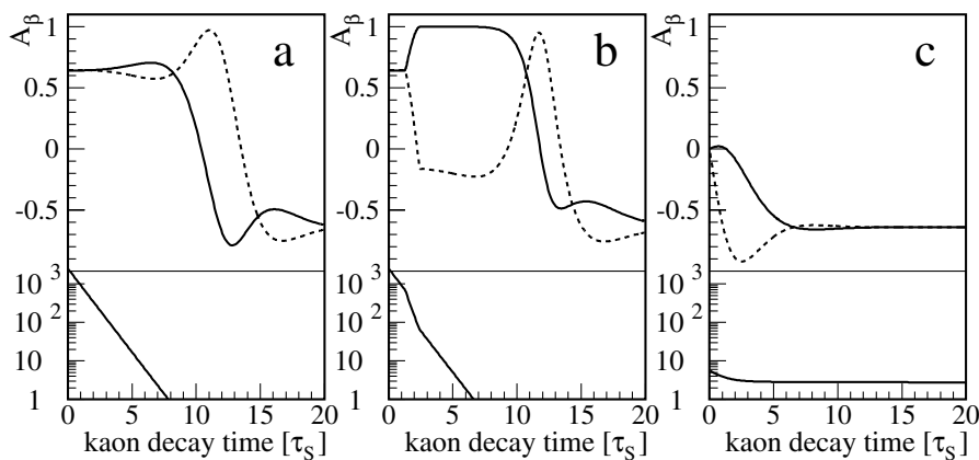
FIG. 2. B^0 - \bar{B}^0 decay rate asymmetries in the \psi K channel as a function of the kaon decay time for various kaon decay final states: (a) 2\pi ; (b) 2\pi with a tungsten regenerator 12 cm thick at a distance of 14 cm; and (c) \pi^- \ell^+ \nu (Kaysers method). The solid (dashed) lines mark the asymmetries for \beta = 70^\circ ( 20^\circ ). A kaon momentum of 2 GeV/c is assumed. To illustrate the statistical requirements we show in the lower thirds of the figures the number of expected decays per \tau_S bin for 10000 B \rightarrow \psi K decays.
