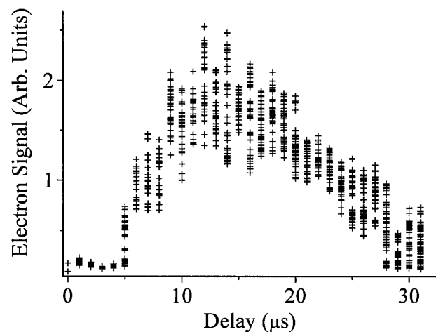
FIG. 3. Electron signal vs delay after excitation of the Cs 39d state, showing that the plasma lives for about 30 \mu\text{s} .
