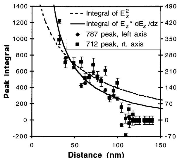
FIG. 2. The points show the integral under the 712\text{ cm}^{-1} peak and that under the 787\text{ cm}^{-1} peak in difference spectra obtained by subtracting spectra at the distances indicated from those far from the surface. The solid line is a model for GFR as described in the text, and the dotted line is what would be expected for the standard Raman case.
