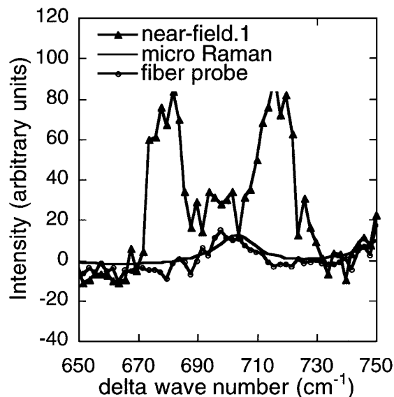
FIG. 1. Scaled (to the peak at 767 \text{cm}^{-1} ) Raman spectra for KTP showing differences between near-field spectra, micro-Raman spectra, and far-field spectra through the probe.
