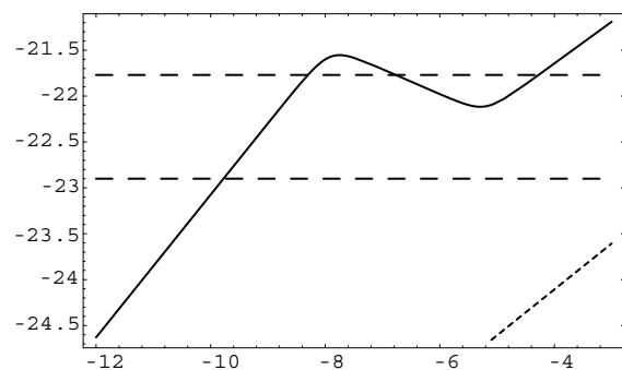
FIG. 1. Gravitational wave amplitude of bursts emitted by cosmic string cusps in the LIGO/VIRGO frequency band, as a function of the parameter \alpha = 50G\mu (in a base-10 log-log plot). The horizontal dashed lines indicate the one sigma noise levels (after optimal filtering) of LIGO 1 (initial detector) and LIGO 2 (advanced configuration). The short-dashed line indicates the rms amplitude of the stochastic GW background.
