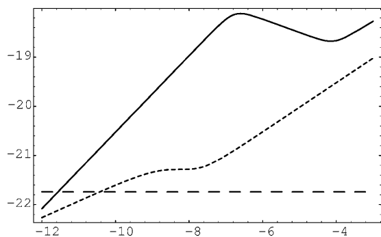
FIG. 2. Gravitational wave amplitude of bursts emitted by cosmic string cusps in the LISA frequency band, as a function of the parameter \alpha = 50G\mu (in a base-10 log-log plot). The short-dashed curve indicates the rms amplitude of the stochastic GW background. The lower long-dashed line indicates the one sigma noise level (after optimal filtering) of LISA.
