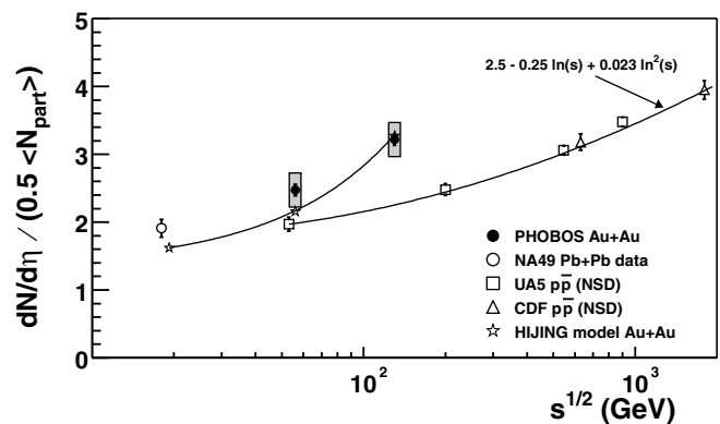
FIG. 4. Measured pseudorapidity density normalized per participant pair for central Au + Au collisions. Systematic errors are shown as shaded area. Data are compared with p\bar{p} data and Pb + Pb data from the CERN SPS. Also shown are results of a HIJING simulation (with a line to guide the eye) and a parametrization of the p\bar{p} data [7].
