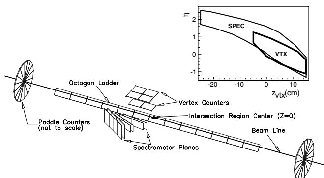
FIG. 1. Detector setup for the initial running period. The inset shows the \eta acceptance of the SPEC and VTX subdetectors as a function of primary vertex position.
