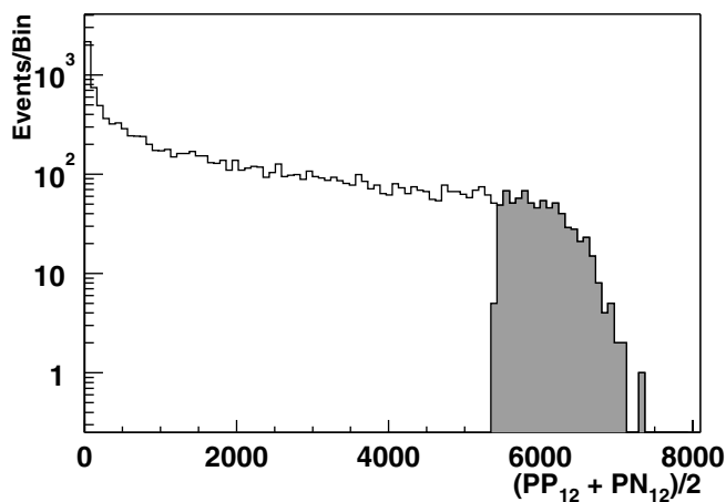
FIG. 2. Paddle signal distribution for data events at \sqrt{s_{NN}} = 130 GeV.
