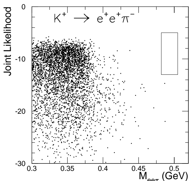
FIG. 6. Similar to Fig. 4, but for K_{ee\pi} .
