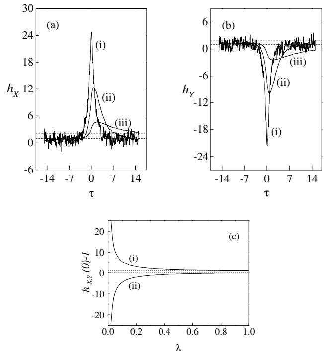
FIG. 2. Quantum trajectory simulation of CHD for the degenerate parametric oscillator: (a) X-quadrature amplitude (unsqueezed), (b) Y-quadrature amplitude (squeezed); with intracavity photon number \langle \hat{a}^\dagger \hat{a} \rangle = 2.0 \times 10^{-4} ( \lambda = 0.02 ), r = 0.5 , N_s = 10000 , and (i) \Gamma = 10 , (ii) \Gamma = 0.5 , and (iii) \Gamma = 0.1 . The dashed lines are the classical bounds. (c) h_x(0) - 1 (i) and h_y(0) - 1 (ii) as a function of \lambda .
