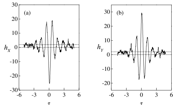
FIG. 3. Quantum trajectory simulation of CHD for single-atom cavity QED: (a) X-quadrature amplitude (in phase with the mean field), (b) Y-quadrature amplitude; with dipole coupling constant g = 6 , atomic decay rate \gamma = 2 , intracavity photon number \langle \hat{a}^\dagger \hat{a} \rangle = 2.8 \times 10^{-4} , r = 0.5 , N_s = 10000 , and \Gamma = 10 . The dashed lines are the classical bounds.
