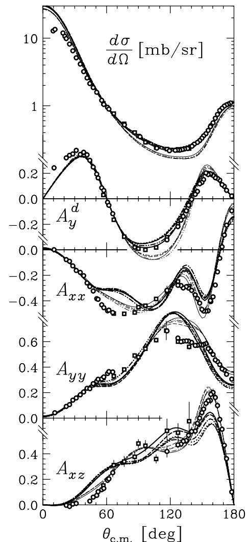
FIG. 1. Angular distributions of cross section and analyzing powers A_y^d , A_{xx} , A_{yy} , and A_{xz} for d p elastic scattering at 270 MeV. Experimental data (open circles and open squares from Ref. [17]) are compared with Faddeev calculations. Only statistical errors are indicated. Thin lines are based on NN forces alone using the CD-Bonn (solid), AV18 (dashed), Nijmegen-I (dotted), Nijmegen-II (dot-dashed), and Nijmegen-93 (dot-dot-dashed). Thick lines include the TM-3NF. The reduced \chi^2 values for \theta_{c.m.} = 50^\circ - 180^\circ with (without) 3NF for CD-Bonn are 16.9(225.2), 2.52(7.71), 31.6(29.8), 12.2(6.03), and 4.93(0.96) for d\sigma/d\Omega , A_y^d , A_{xx} , A_{yy} , and A_{xz} , respectively. Other NN forces give similar values.
