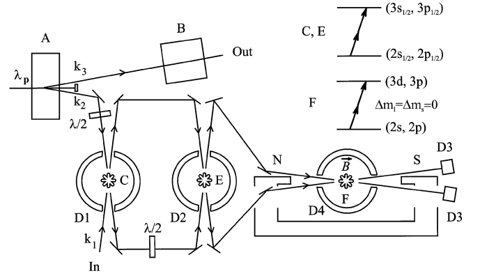
FIG. 1. Total optical teleportation scheme: (A) PDC event; (B) linear polarization rotator; (C,E) singlet-selecting two-photon absorptions; (F) two-photon \Delta m_s = \Delta m_l = 0 absorption event (Zeeman configuration); (D1–D4) single photon detectors.
